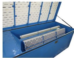
3696 with HDPE Plastic top, Odor eliminating Carbon filters, and Jack bolts under the top for creating an extreme flat work surface for gluing plastics
